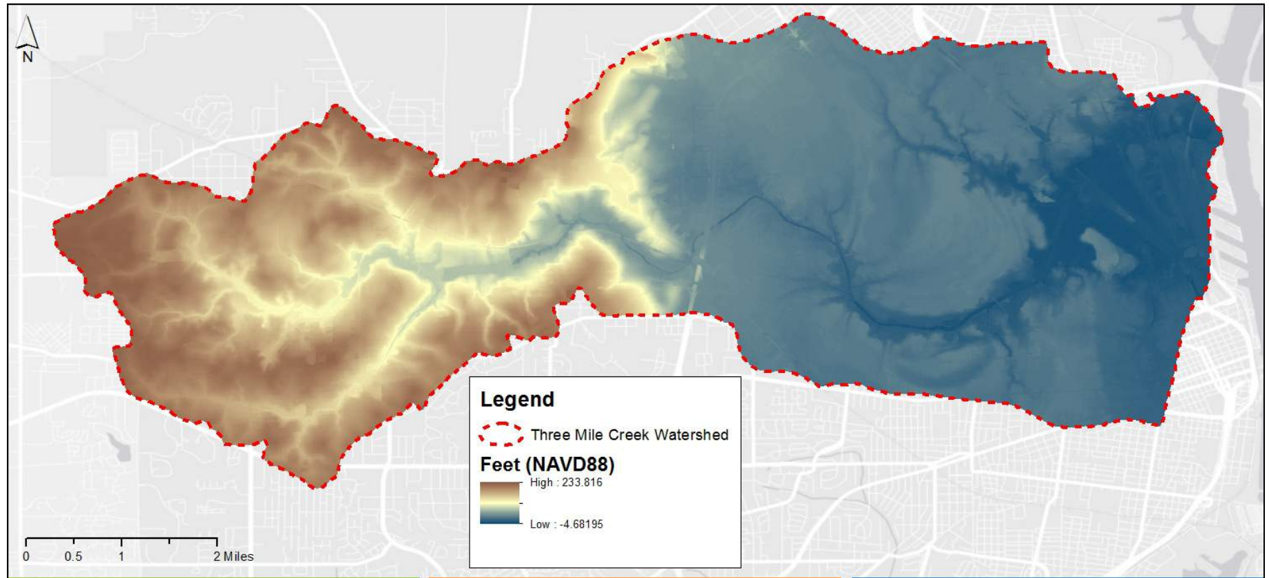
Figure 2-4 The Topography in the Three Mile Creek Watershed has an Abrupt Elevation Change Near I-65 (Source: Mobile County LiDAR, 2002)
